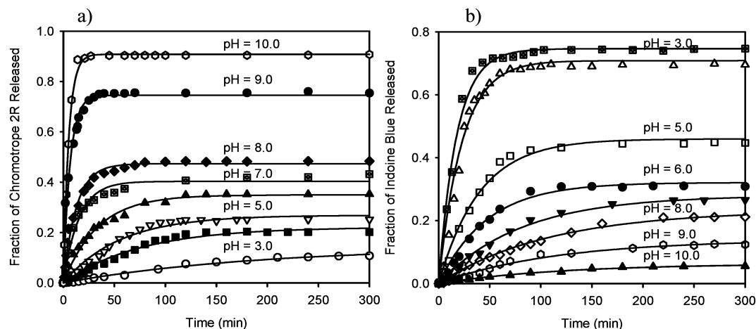
Figure 7. Release profiles for (a) Chromotrope 2R and (b) Indoine Blue as a function of solution pH from (PAH/HA) 10 multilayer films assembled at pH = 3.0. Loading pH = 9.0 for Indoine Blue and pH = 3.0 for Chromotrope 2R.
