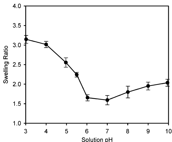
Figure 3. Ratio of the equilibrium swelling thickness to the dry film thickness for (PAH/HA) 10 films assembled at pH = 3.0 exposed to different solution pH values.
