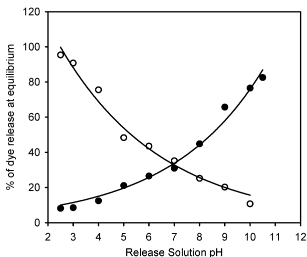
Figure 8. Total percentage of incorporated Chromotrope 2R (●) and Indoine Blue (○) released under equilibrium conditions from the (PAH/HA) 10 films at different solution pH values.
