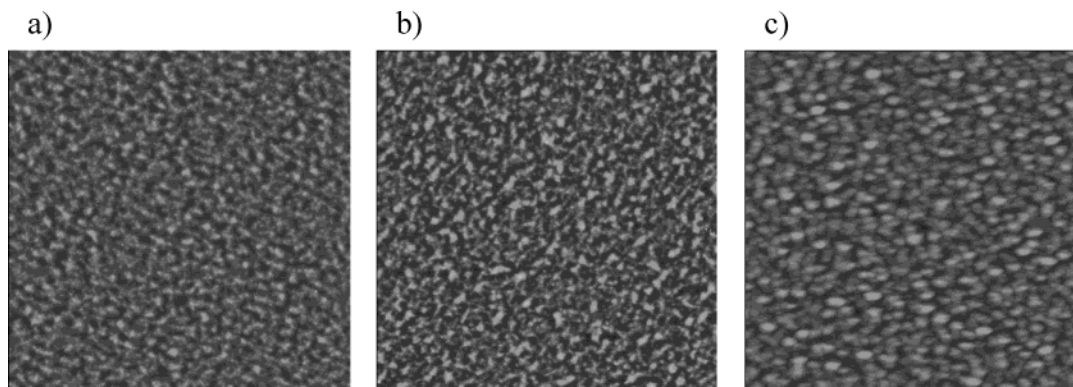
Figure 4. AFM ( 25 \times 25 \mu\text{m} ) height images of (\text{PAH/HA})_{10} multilayer films assembled at pH = 3.0: (a) before exposure to solution (rms = 5.3 nm), (b) after exposure to pH = 3.0 (rms = 7.2 nm), (c) after exposure to pH = 10.0 (rms = 11.6 nm).
