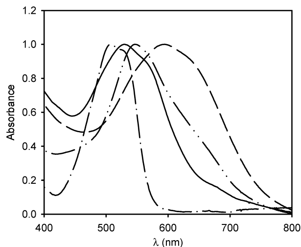
Figure 6. Normalized absorbance spectra of Chromotrope 2R in solution (— · —), Chromotrope 2R in a (PAH/HA) 10 film (—), Indoine Blue in solution (— · · —), and Indoine Blue in a (PAH/HA) 10 film (— —).
