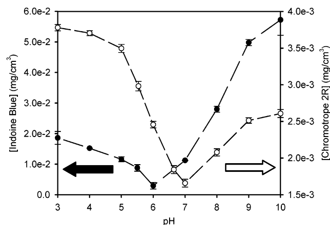
Figure 5. Concentration of dye molecules incorporated into (\text{PAH/HA})_{10} multilayer films assembled at pH = 3.0 as a function of the solution pH: Indoine Blue (●) and Chromotrope 2R (○).
