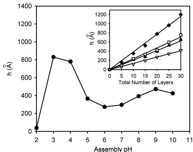
Figure 2. Dependence of (PAH/HA) 10 film thickness on the assembly solution pH. Insert plot shows the linear growth of PAH/HA films as the total number of layers is increased for films assembled at pH = 4.0 (◆), pH = 6.0 (▽), pH = 8.0 (▲), and pH = 10.0 (□). Error in thickness of \pm 5 –16 Å.
